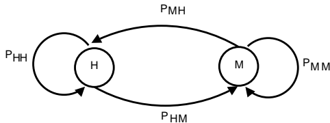
Fig. 3. Attack Model.
